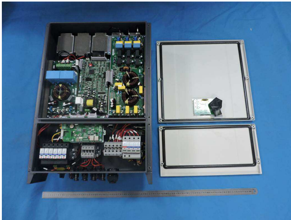
Internal view-1
