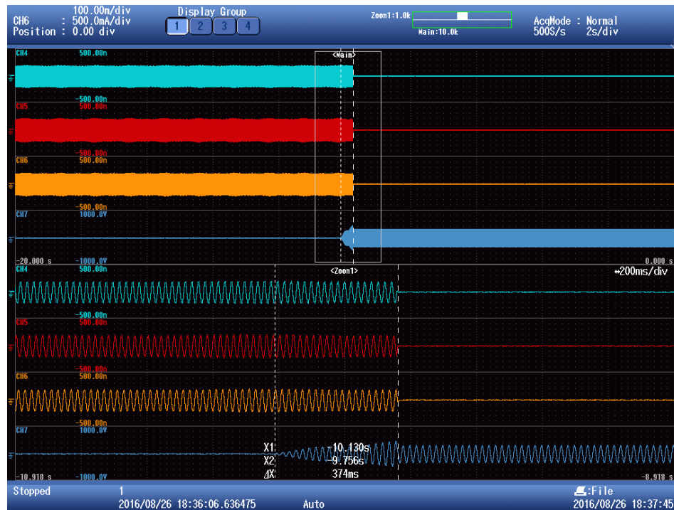
CH4,CH5, CH6: EUT output current; CH7: trip signal of switch off;
