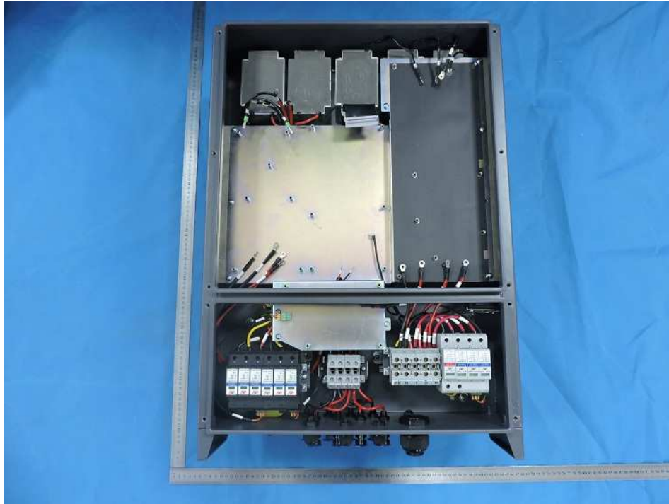
Internal view-3
